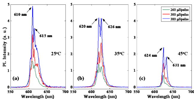
FIG. 2. (Color online) Lasing spectra measured along \Gamma M direction at temperatures of (a) 25 °C, (b) 35 °C, and (c) 45 °C, under different pumping energies of 260, 300, and 380 \mu\text{J}/\text{pulse} .
