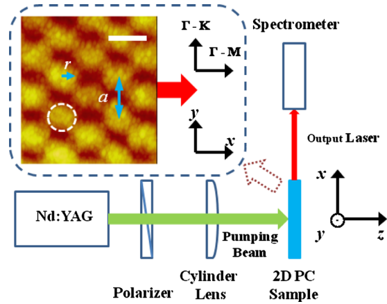
FIG. 1. (Color online) Schematic optical setup of the lasing experiment. Inset figure is an AFM image for the surface morphology of a 2D hexagonal H-PDLC PC. Scale bar: 500 nm.
