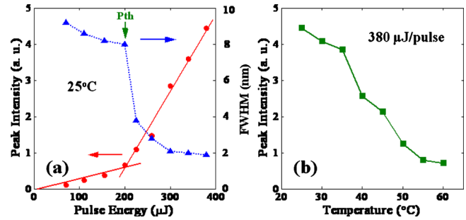
FIG. 3. (Color online) (a) Dependences of peak intensity and FWHM of PL maximum peak on pumping energy at 25 °C. The threshold of pumping energy ( P_{th} ) is around 200 \mu\text{J}/\text{pulse} . (b) Dependence of lasing peak intensity on temperature. The pumping energy is 380 \mu\text{J}/\text{pulse} .
