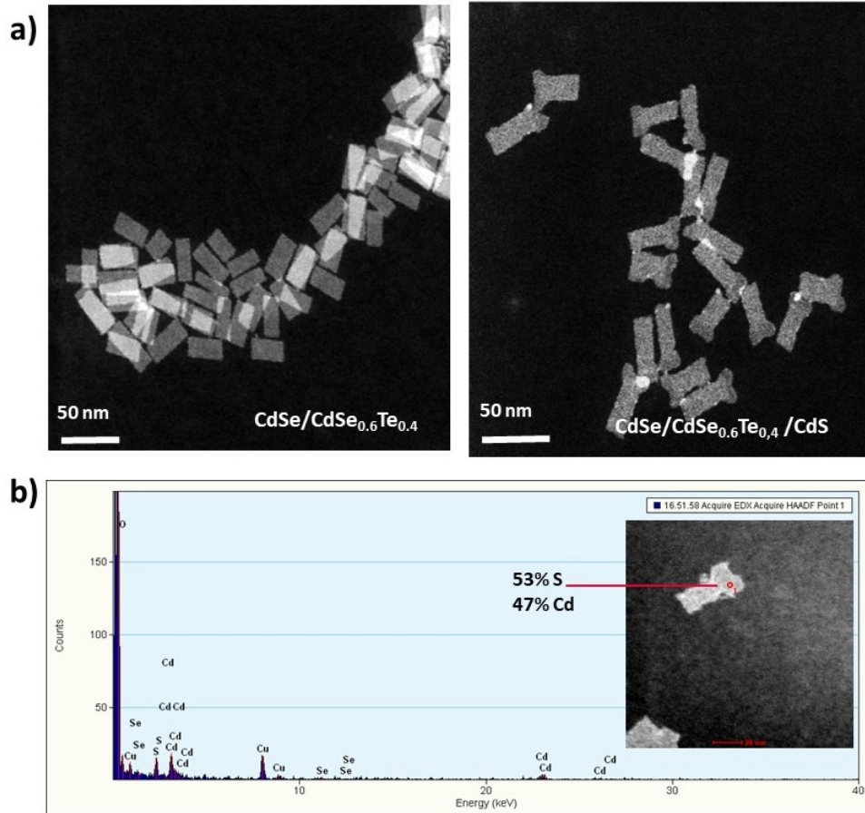
Figure 5.14: (a)HAADF-TEM image of 4 ML CdSe/Cd Se_{0.6}Te_{0.4} core/alloved-crown and CdS-coated core/alloved-crown/crown NPLs and (b) EDX analysis performed on CdSe/Cd Se_{0.6}Te_{0.4} /CdS core/alloved-crown/crown NPLs. CdS formation is verified.
