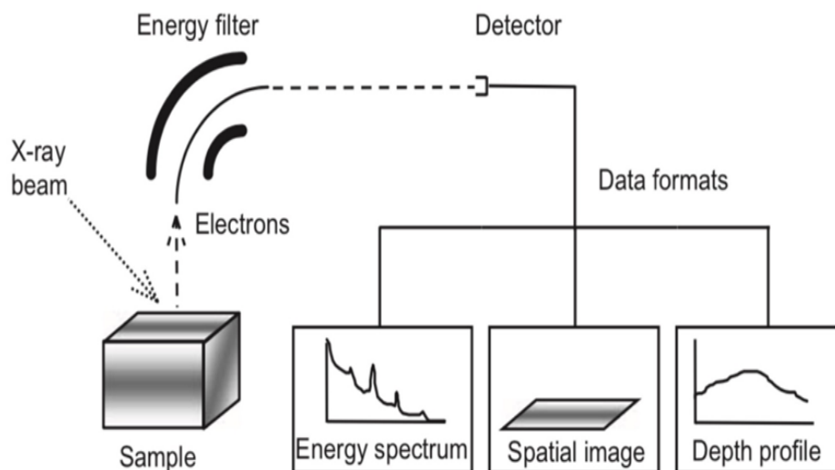
Figure 3.10: Schematic representation of XPS. Reprinted with permission from [2].
