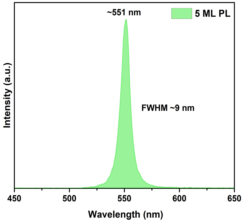
Figure 3.4: PL spectrum of 5 ML thick NPLs.
