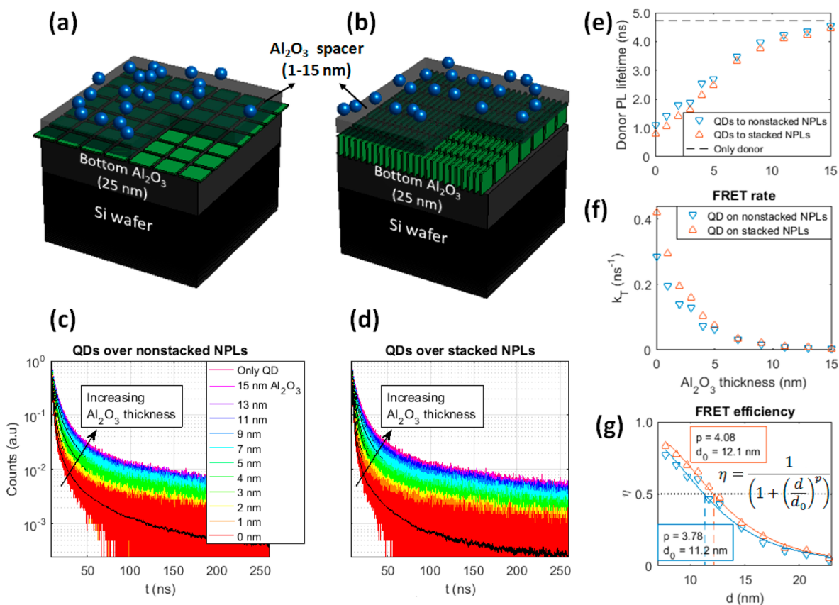
Figure 4. Film structure for distance-dependent FRET from the QDs to (a) the nonstacked NPLs and (b) the stacked NPLs. The spacer thickness is varied from 1 to 15 nm. PL decays of QDs over (c) the nonstacked NPLs and (d) the stacked NPLs for tuned spacer thicknesses. The black curves are multiexponential fits to PL decays convolved with the instrument response function. (e) The resulting PL lifetimes of QDs and (f) extracted rates of FRET to the nonstacked (blue down triangles) and the stacked NPLs (orange up triangles). (g) FRET efficiencies as a function of the donor–acceptor distance along with their numerical fits to the FRET efficiency formula in the inset (eq 4). The data captures the d^{-4} behavior in general for both the nonstacked and stacked NPLs. The horizontal dashed lines indicate the Förster distances for FRET to the nonstacked (blue) and stacked (orange) NPLs.
