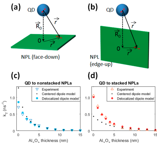
Figure 5. Variation of distance between a QD dipole and an NPL dipole for (a) nonstacked and (b) stacked NPL orientation, depending on the position \vec{r}' of the NPL dipole state. (c) Experimental rates of FRET to the nonstacked NPL monolayer (blue down triangle) compared to those estimated by two different models based on Förster's theory: center-to-center distance approach (small black dots) and delocalized dipole approach (large blue dots). (d) Experimental rates of FRET to the stacked NPL monolayer (orange up triangle) compared to the those estimated by center-to-center distance approach (small black dots) and delocalized dipole approach (large red dots). The delocalized dipole approach shows an excellent agreement with the experimental data whereas the centered dipole approach yields increasing discrepancy as the spacer thickness is diminishing.
