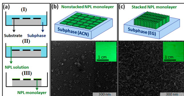
Figure 2. (a) Liquid–air interface self-assembly procedure: (I) Blank substrates are placed inside the subphase. (II) NPL solution is poured onto the subphase and is then allowed to dry. (III) The subphase is subsequently drained after the evaporation of the NPL solution. Finally, the residual subphase on the substrates is evaporated. NPL orientation on the liquid–air interface depends on the subphase. Schematic representation of NPL monolayers (b) on acetonitrile (ACN) and (c) on ethylene glycol (EG), along with SEM images of these films after being transferred to a solid substrate. The scale bars of the SEM images are 300 nm. ACN results in nonstacked self-assembly, whereas EG results in stack formation. Insets in the SEM images show real-color fluorescence images of the resulting monolayer assemblies on wafers of thermal oxide with scale bars of 1 cm.
