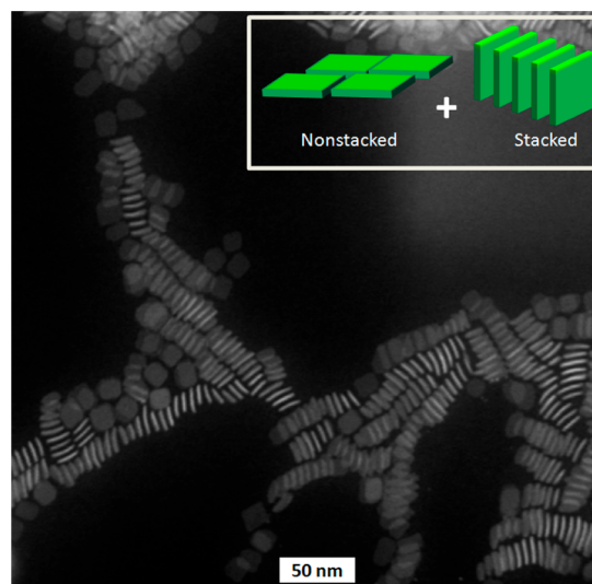
Figure 1. High-angle annular dark-field scanning transmission electron microscopy (HAADF-STEM) image of 4 ML CdSe NPLs. Inset schematically shows the orientation of nonstacked (face-down) and stacked (edge-up) NPLs in three dimensions with the imaged facets highlighted in light green.
