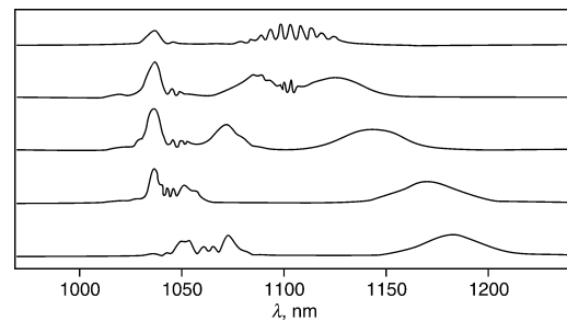
Fig. 2 Wavelength tuning with input polarisation control
