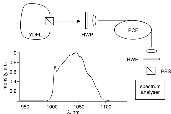
Fig. 1 Experimental configuration and typical output spectrum from ytterbium-doped fibre laser (YDFL)
