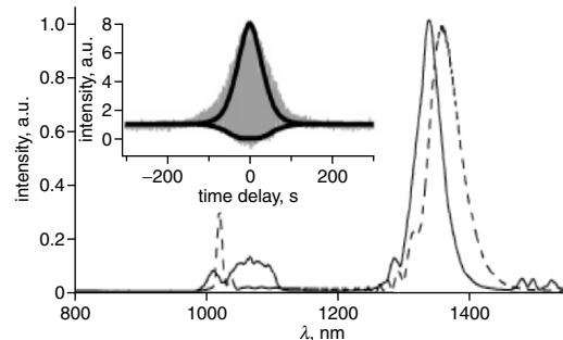
Fig. 3 Measured spectrum of pulse at 1.33 \mu\text{m} and result from numerical simulation
