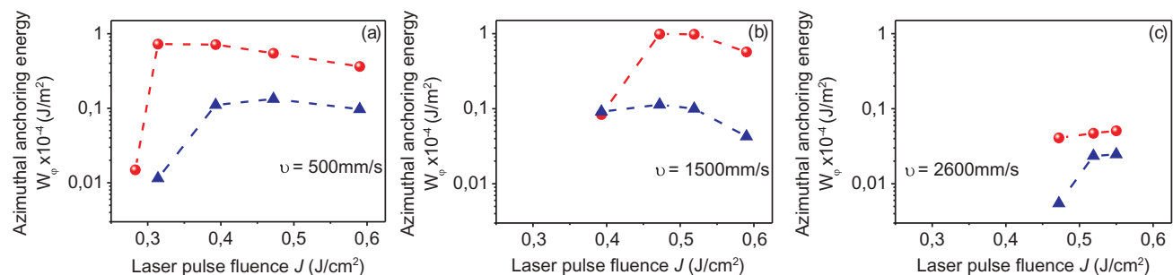
Figure 4. (Colour online) Dependence of the calculated azimuthal AE (Equation (2)) of aligning films on the LPF J at constant scanning speed v : (a) 500 mm/s, (b) 1500 mm/s and (c) 2600 mm/s during the processing of the Ti layer with the NLL method. The LC cell consists of the tested substrate having the pure NSTL (closed 'blue' triangles) and NSTL coated with the ODAPI film (closed 'red' spheres). The dashed line is a guide to the eye.
